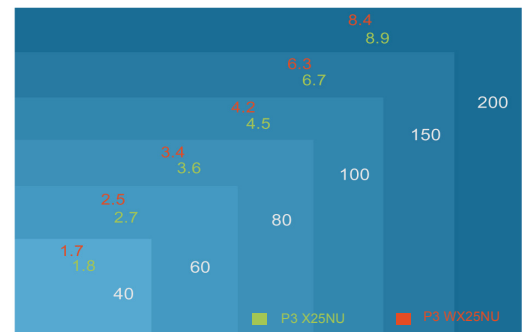
Note: allow 3-5% variance on all projector throw ratios
